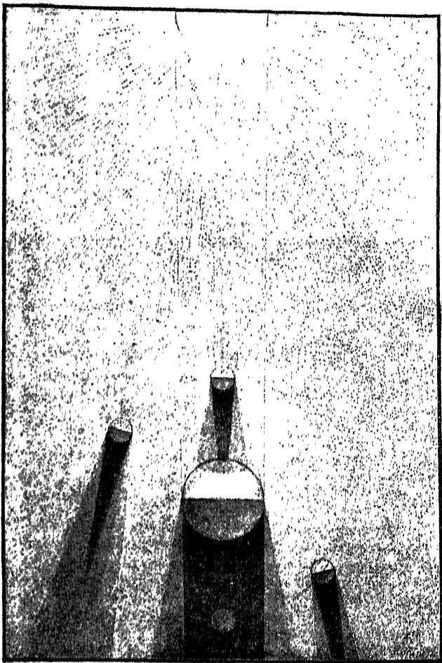
TO SHOW HOW ECLIPSES TAKE PLACE
